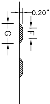
TRUNCATED DOME DETECTABLE WARNING DETAIL
