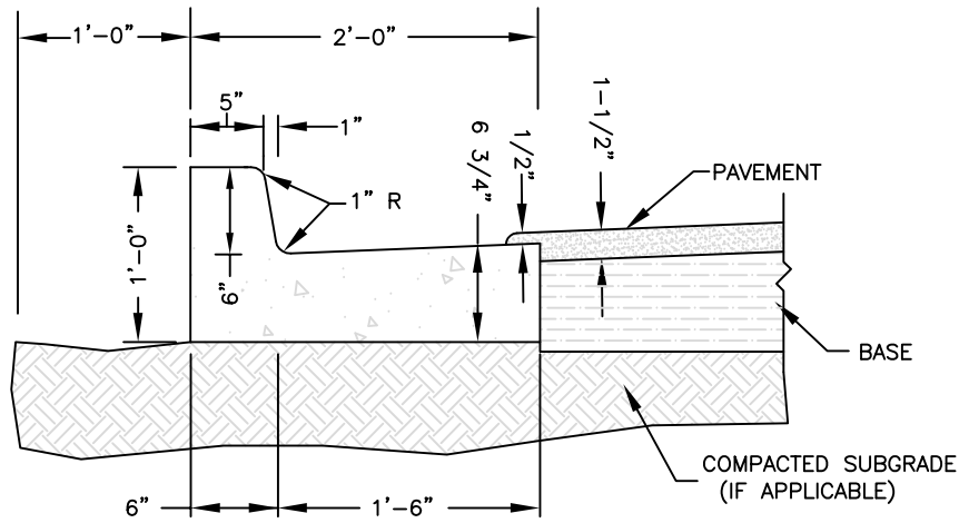
CURB & GUTTER DETAIL NOT TO SCALE
