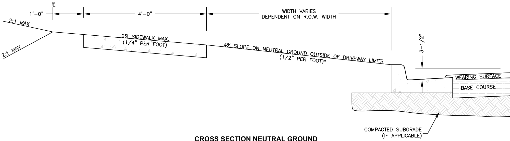
CROSS SECTION NEUTRAL GROUND NOT TO SCALE
